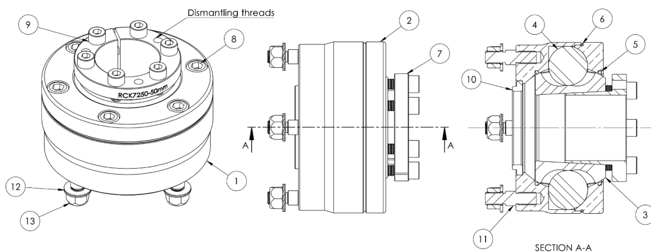
Fig 4. Parts Diagram
